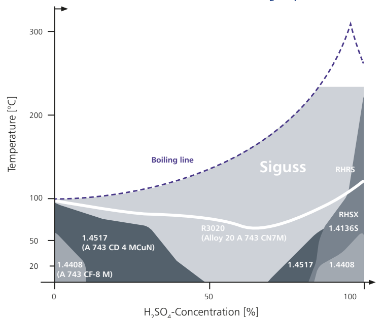
ISO Corrosion diagram for materials in H_2SO_4
