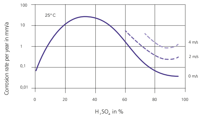
Influence of flow rate of H_2SO_4 on the corrosion rate for 1.4408
